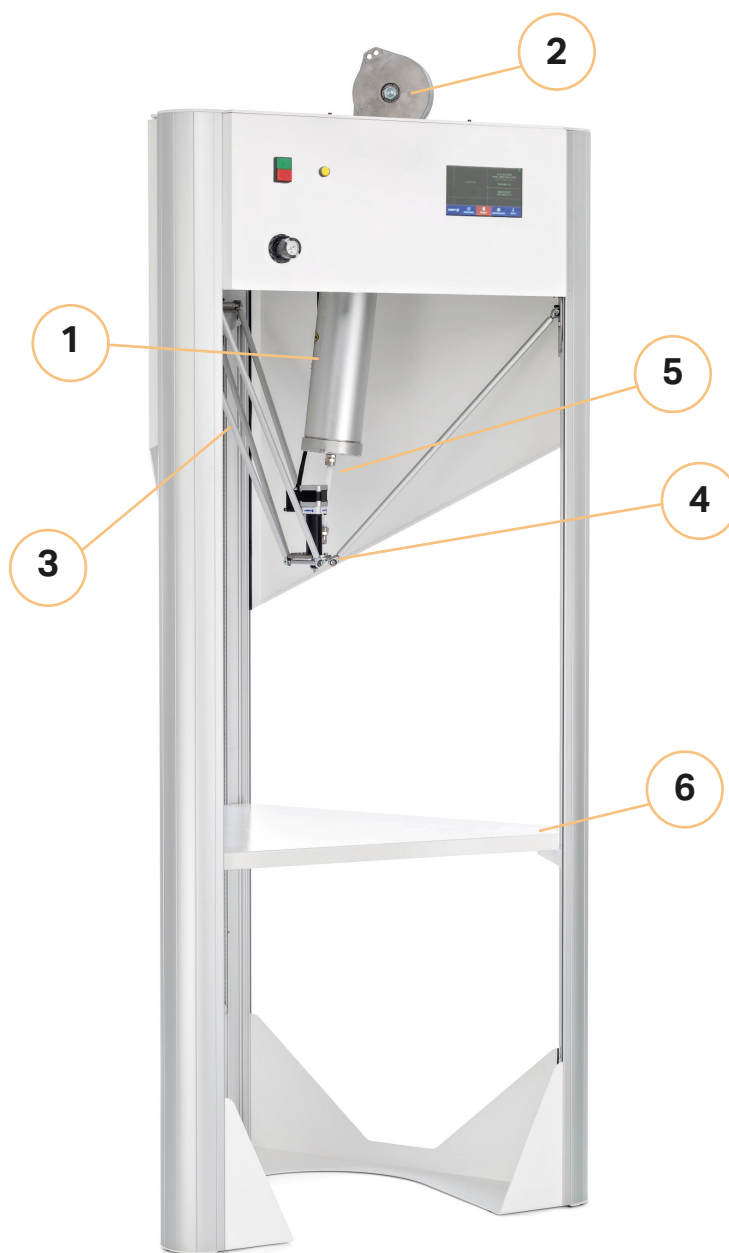
Fig. 2.2 - Working zone
